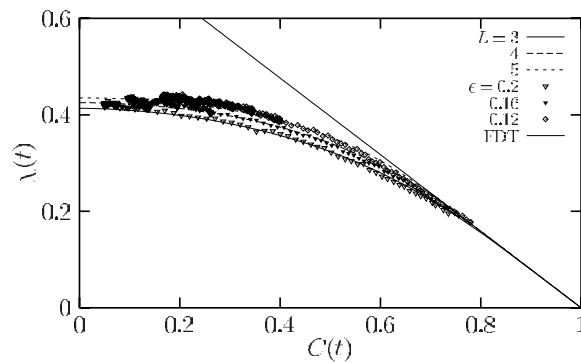
Figure 3. Test of the static–dynamic relationship (15) for the driven dynamics for d = 4 and T = 0.7T_c . The points are dynamic FD plots, the lines are the double integral of the Parisi function measured in equilibrium simulations.
